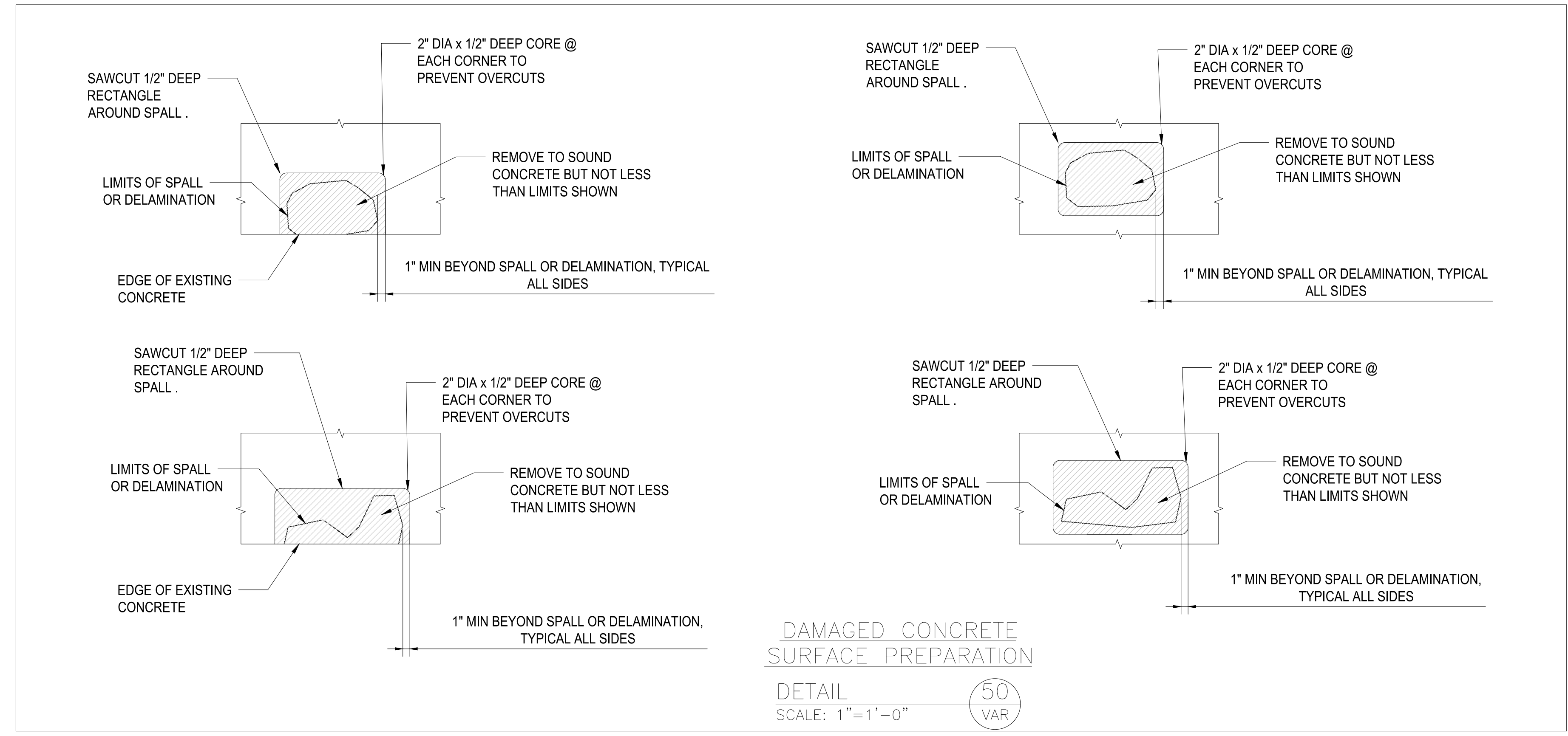
DEEP SPALL REPAIR WITH DAMAGED REBAR DETAIL 49 SCALE: 1"=1'-0" VAR
