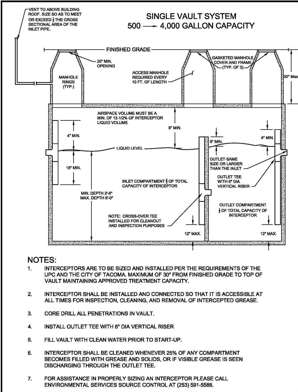
Figure 5-2: Single Vault Gravity Grease Interceptor
