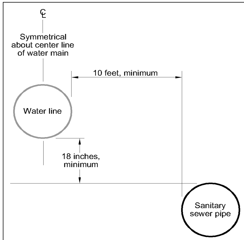
Figure 3-1: Minimum Separation
