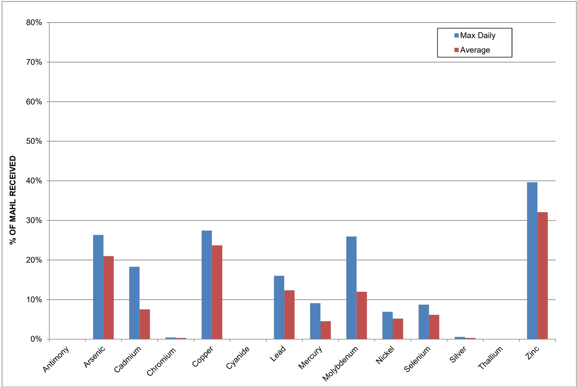
Figure 4-1 A Comparison of 2014 CTP Loadings and Calculated MAHL
