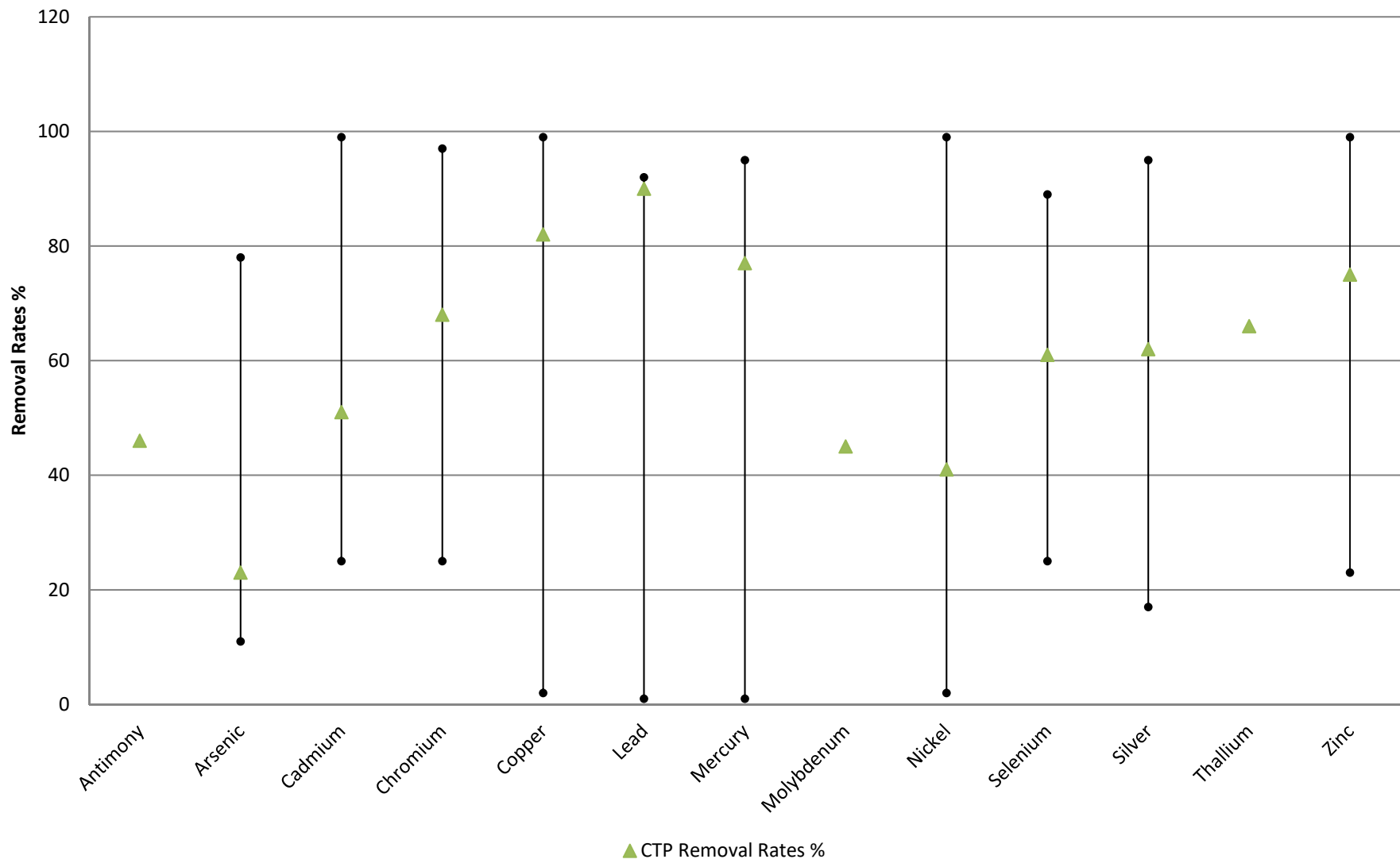
Figure 3-2 CTP Removal Rates and the range of standard Removal Rates presented by EPA
